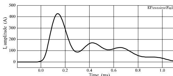
Figure 2. A typical transient earth fault current pulse
