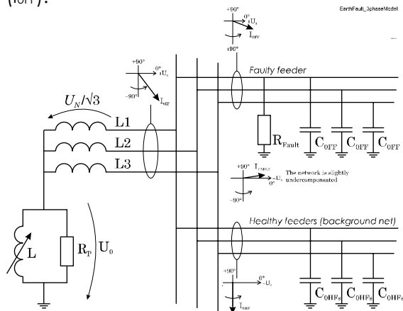
Figure 1. Compensated network
