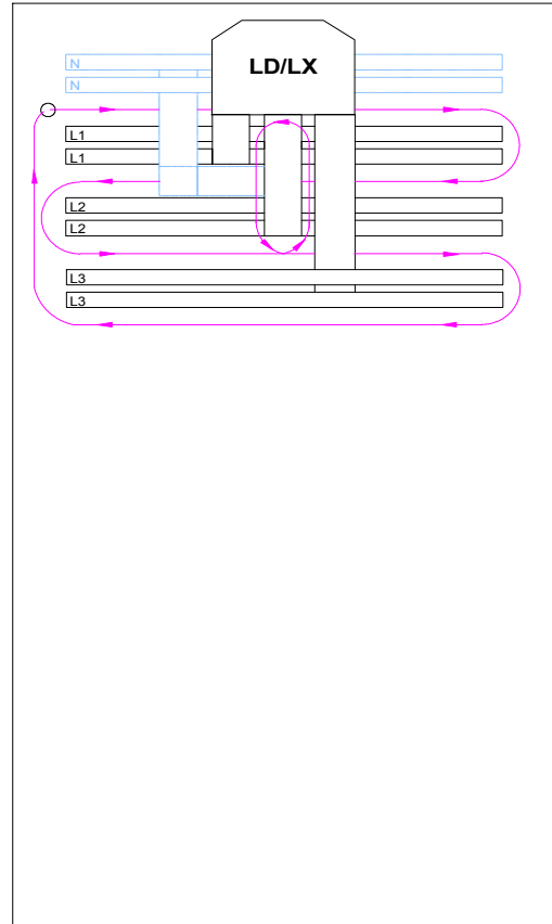
LD/LX-Connection system Type A
